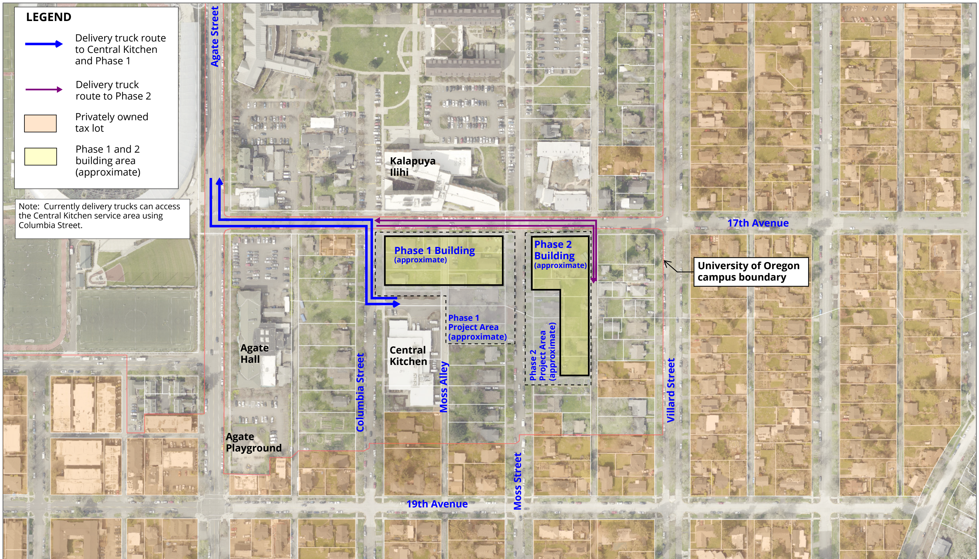
East Campus Delivery Truck Circulation (Box Trucks) Diagram 3-14-25
